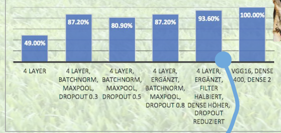
Test Accuracy
