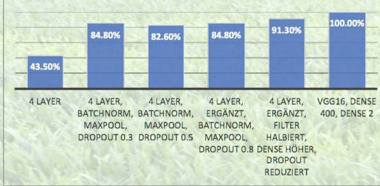
Validation Accuracy
